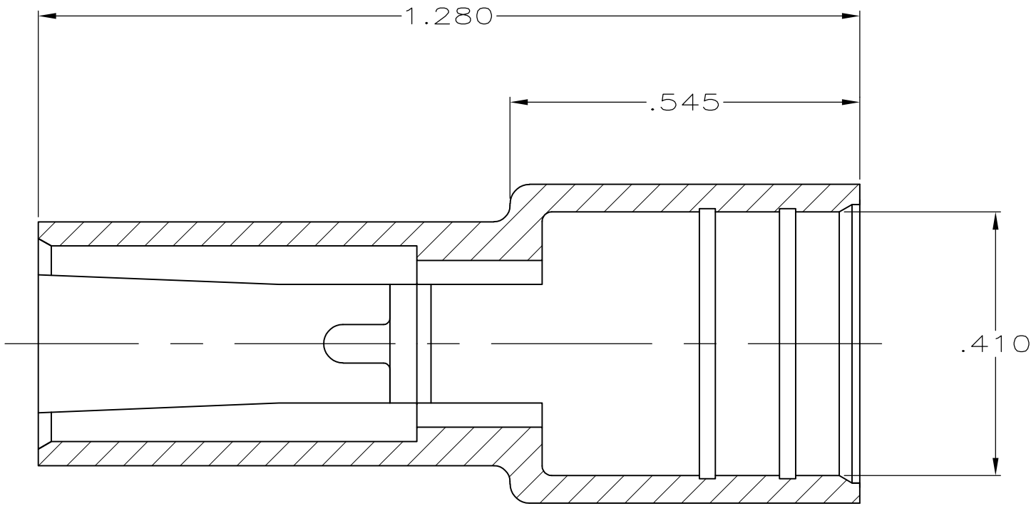
SECTION X-X
