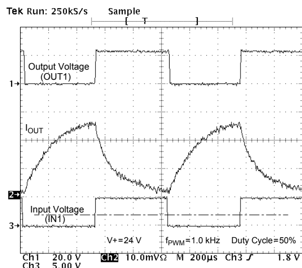
Figure 11. Output Voltage and Current vs. Input Voltage at V+ = 24\ \text{V} , PWM Frequency of 1.0 kHz, and Duty Cycle of 50%
