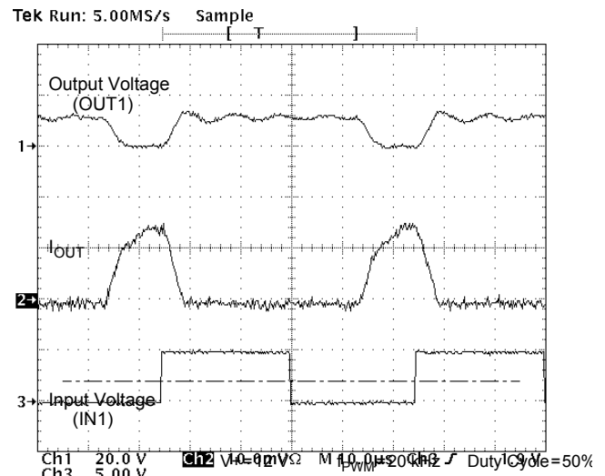
Figure 16. Output Voltage and Current vs. Input Voltage at V + = 12 V, PWM Frequency of 20 kHz, and Duty Cycle of 50% for a Purely Resistive Load
