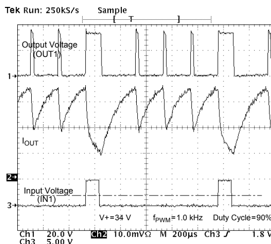
Figure 12. Output Voltage and Current vs. Input Voltage at V+ = 34\ \text{V} , PWM Frequency of 1.0 kHz, and Duty Cycle of 90%, Showing Device in Current Limiting Mode
