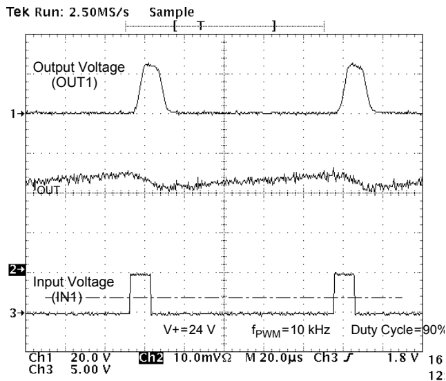
Figure 15. Output Voltage and Current vs. Input Voltage at V + = 24 V, PWM Frequency of 10 kHz, and Duty Cycle of 90%
