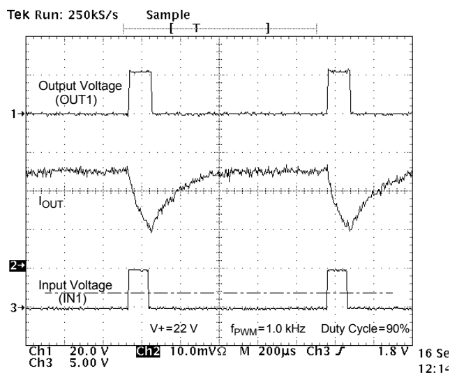
Figure 13. Output Voltage and Current vs. Input Voltage at V+ = 22\ \text{V} , PWM Frequency of 1.0 kHz, and Duty Cycle of 90%
