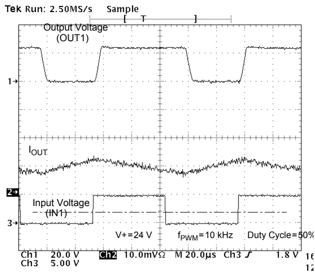
Figure 14. Output Voltage and Current vs. Input Voltage at V + = 24 V, PWM Frequency of 10 kHz, and Duty Cycle of 50%
