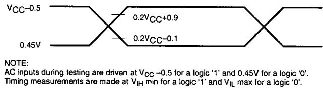
Figure 6. AC Testing Input/Output
