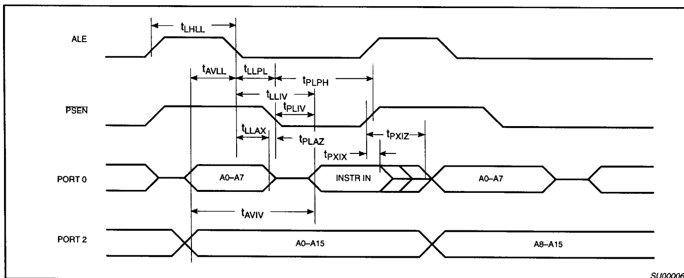
Figure 1. External Program Memory Read Cycle
