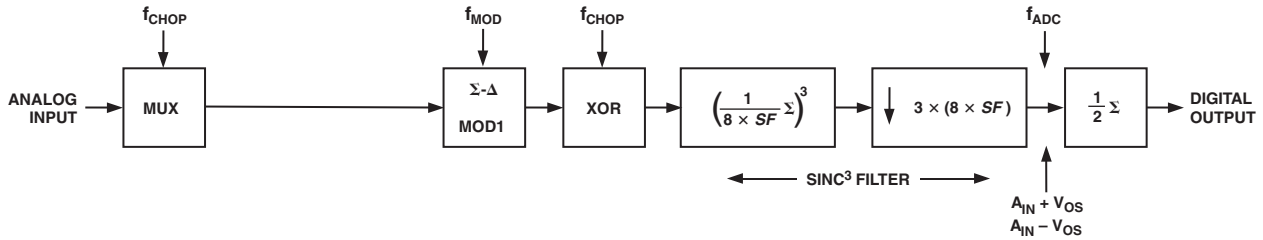
Figure 5. Auxiliary ADC Channel Block Diagram
