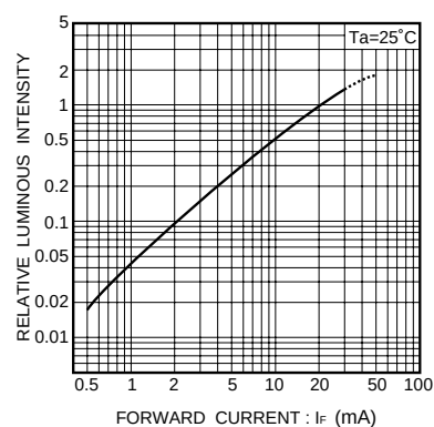
Fig. 4 Luminous intensity vs. forward current
