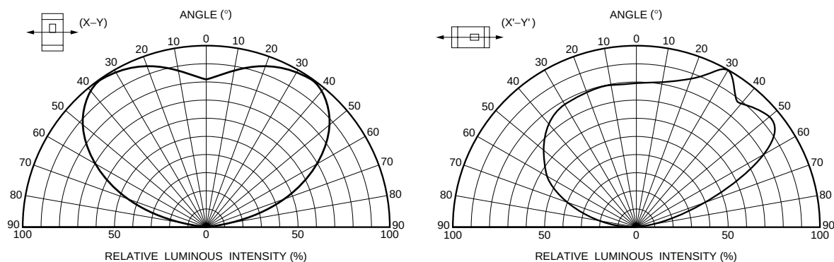
Fig.1 Directional pattern
