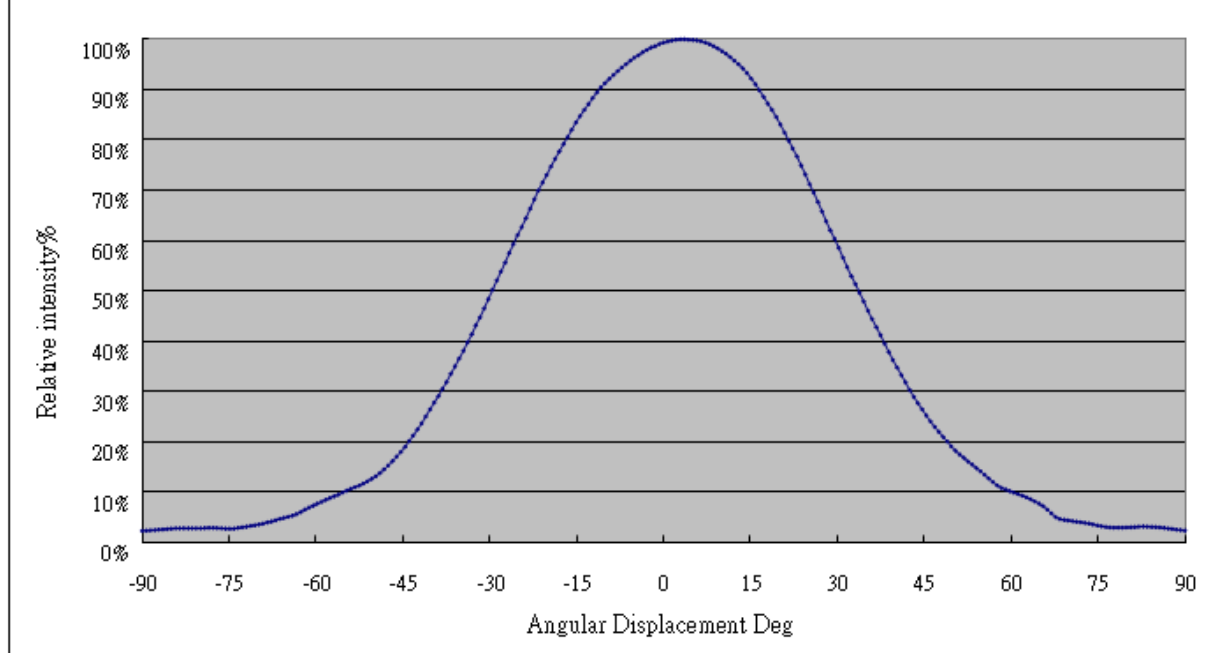
Typical spatial Radiation Pattern
