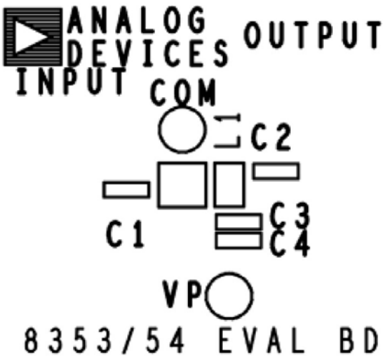
Figure 41. Silkscreen Top
