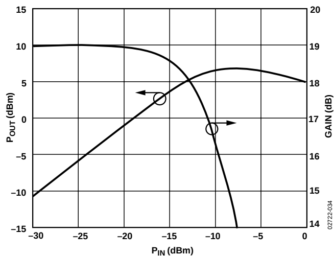
Figure 35. Output Power and Gain vs. Input Power, V_S = 3\text{ V} , T_A = 25^\circ\text{C} , f = 900\text{ MHz}
