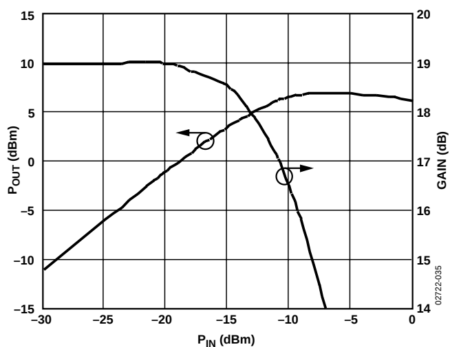
Figure 36. Output Power and Gain vs. Input Power, V_S = 5\text{ V} , T_A = 25^\circ\text{C} , f = 900\text{ MHz}
