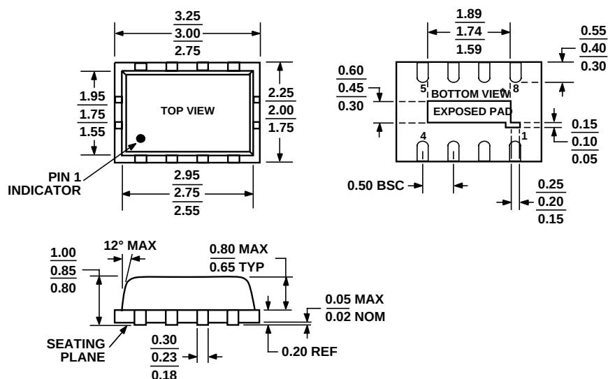
Figure 43. 8-Lead Lead Frame Chip Scale Package [LFCSP_VD] 2 mm × 3 mm Body, Very Thin, Dual Lead CP-8-1
