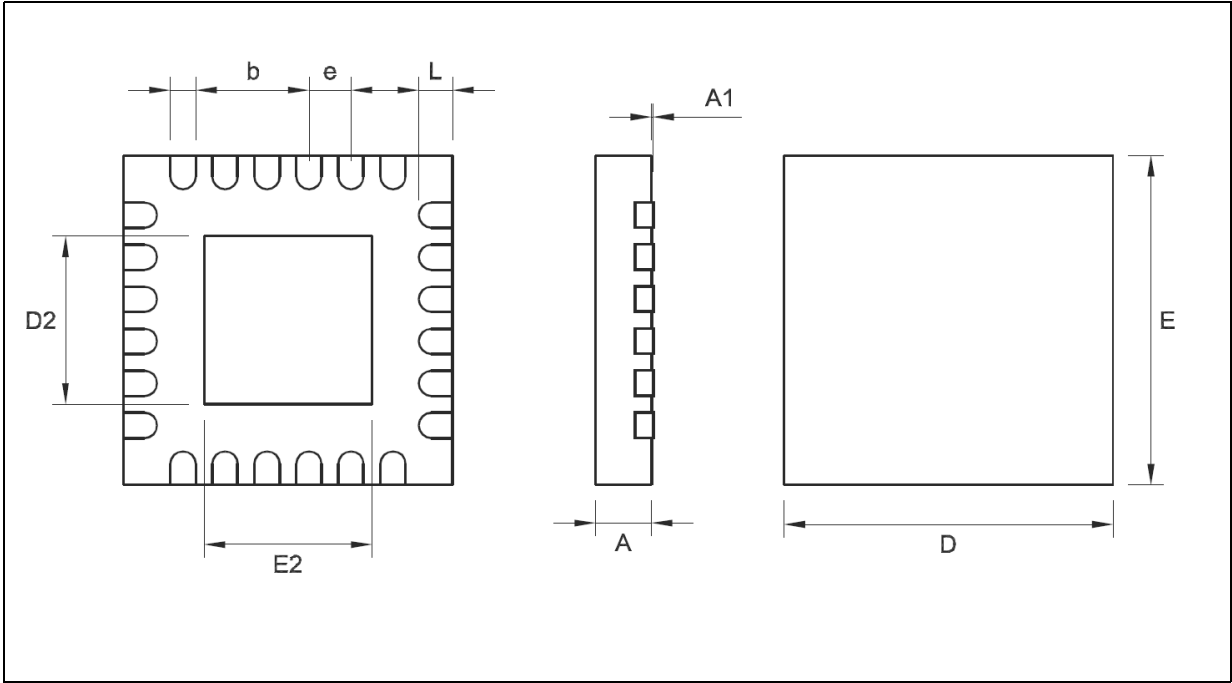
Figure 43. Package dimensions
