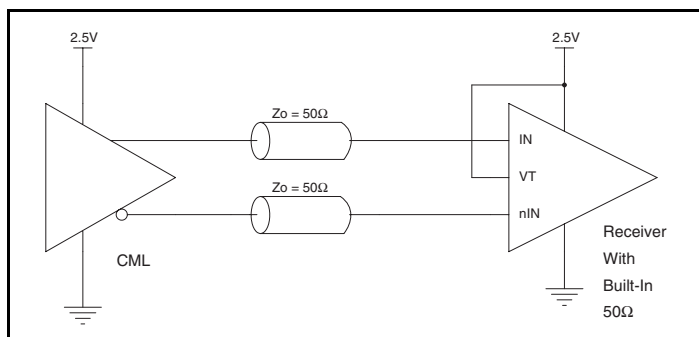
Figure 3C. HiPerClockS IN/nIN Input with Built-In 50 \Omega Driven by a CML Driver
