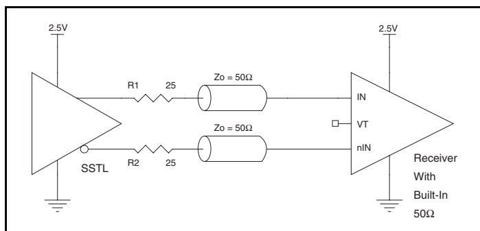
Figure 3E. HiPerClockS IN/nIN Input with Built-In 50 \Omega Driven by an SSTL Driver
