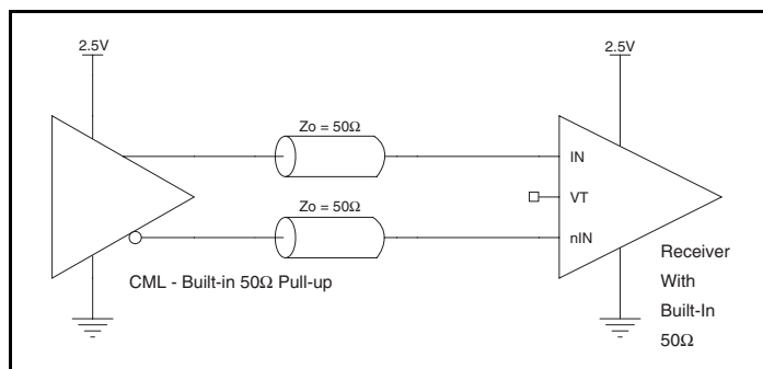
Figure 3D. HiPerClockS IN/nIN Input with Built-In 50 \Omega Driven by a CML Driver with Built-In 50 \Omega Pullup
