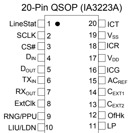
Figure 35. Pin Configuration
