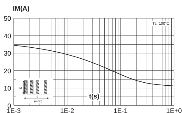
Fig. 4-1: Non repetitive surge peak forward current versus overload duration (TO-220FPAC)
