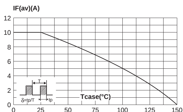
Fig. 2-1: Average current versus case temperature ( \delta = 0.5 ) (TO-220FPAC)
