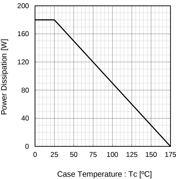
Fig.6 Power Dissipation
