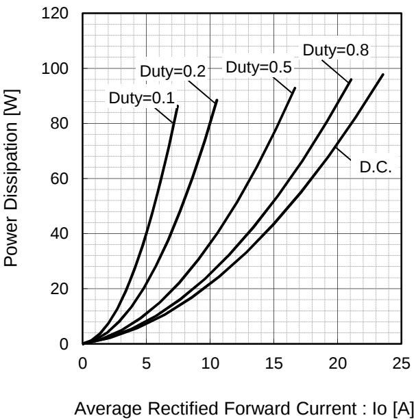
Fig.8 Io-Pf Characteristics
