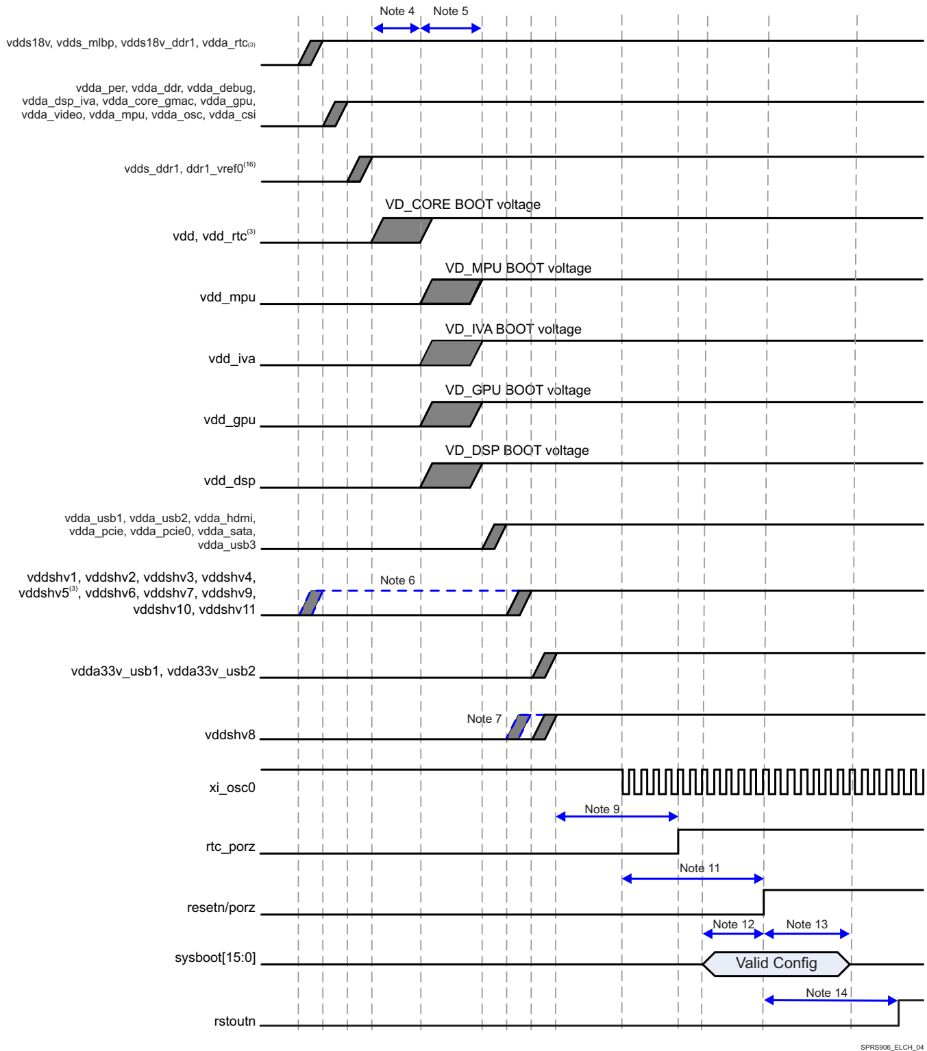
Figure 5-1. Power-Up Sequencing
