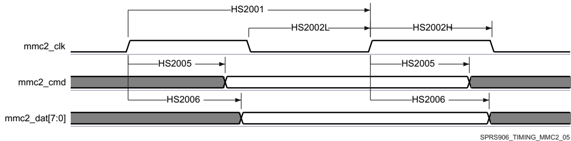
Figure 7-79. eMMC in - HS200 SDR - Transmitter Mode
