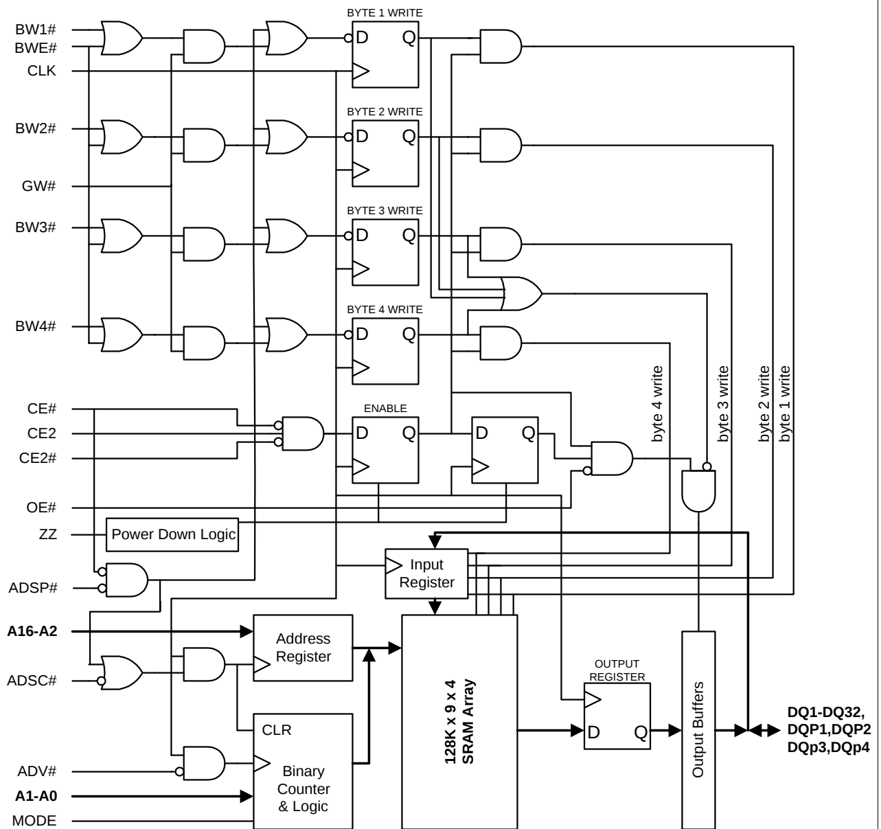
128K x 36 (CY7C1347A/GVT71128G36) Functional Block Diagram [1]
