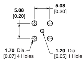
Mounting Detail
