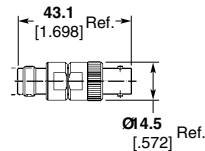
TNC Jack – BNC Jack
