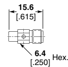
MCX Jack – SMA Jack
