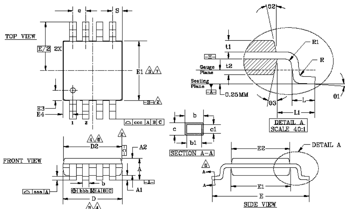
Figure 8. MSOP-8 Package
