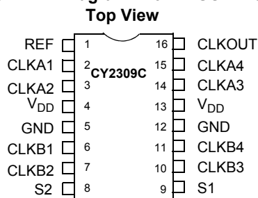
Figure 2. Pin Diagram - 16 Pin SOIC/TSSOP
