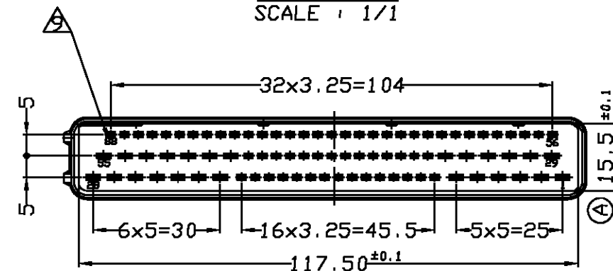
SECTION C-C SCALE : 1/1
