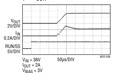
36VIN Start-Up Waveforms (3.3V OUT )
