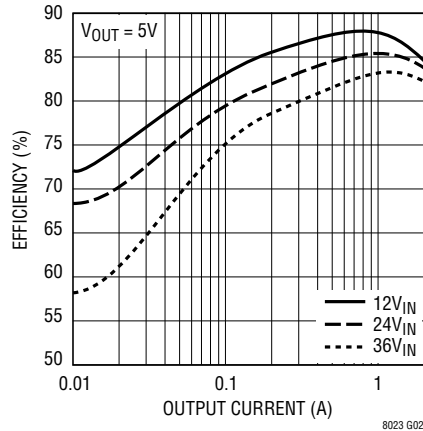
Efficiency (5V OUT )
