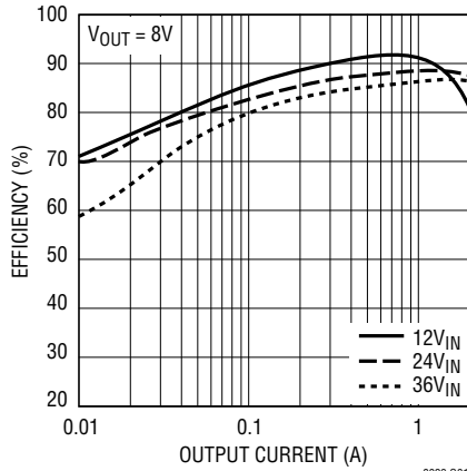
Efficiency (8V OUT )
