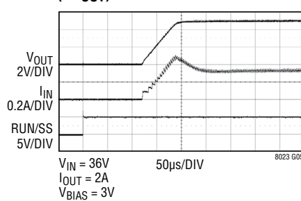
36VIN Start-Up Waveforms (5V OUT )
