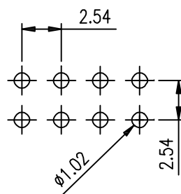
Recommended P.C.Board Hole Layout
