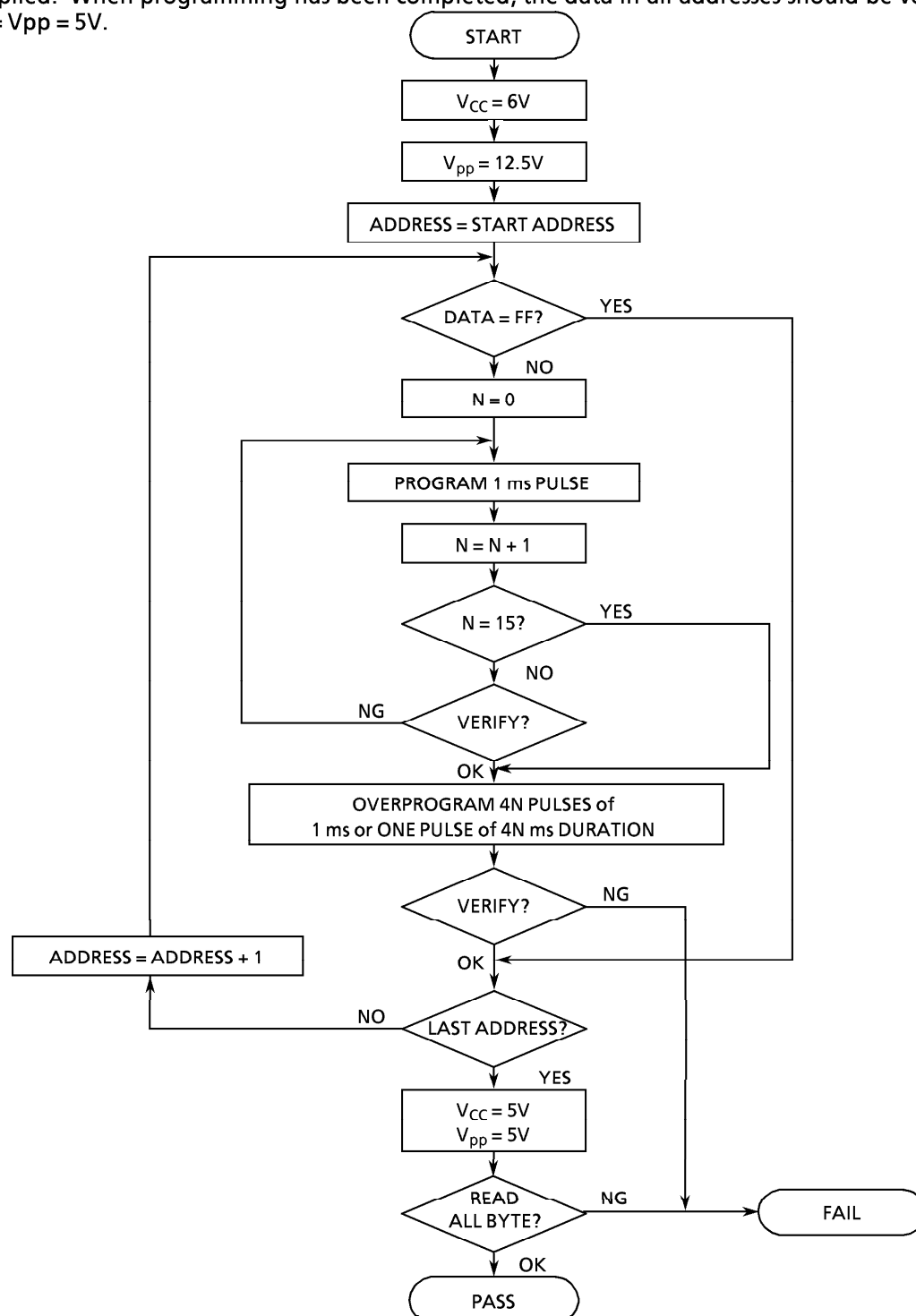
Figure1-4. FLOW CHART
