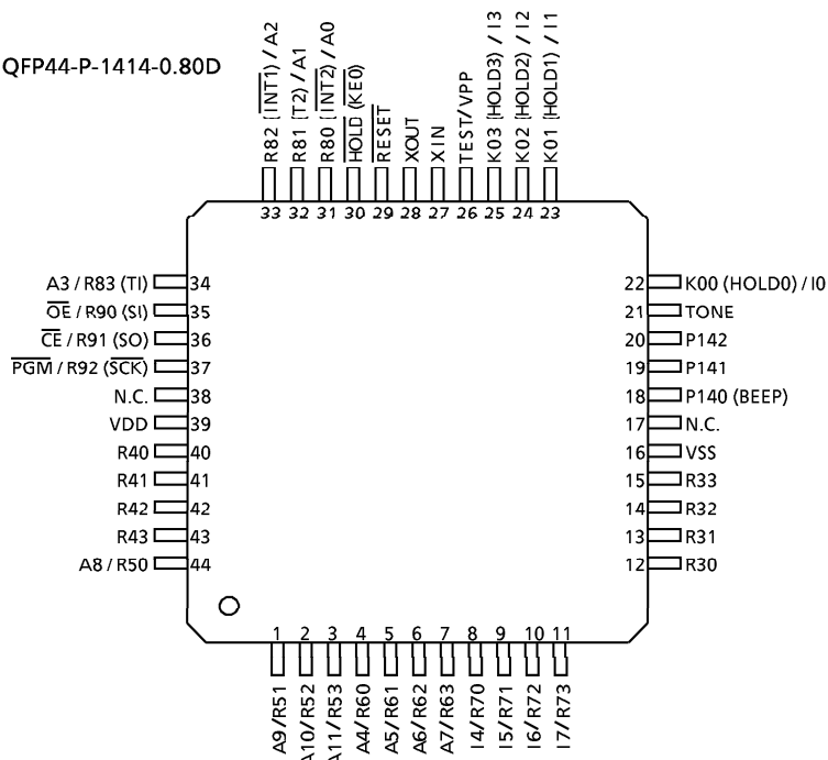
QFP44-P-1414-0.80D
