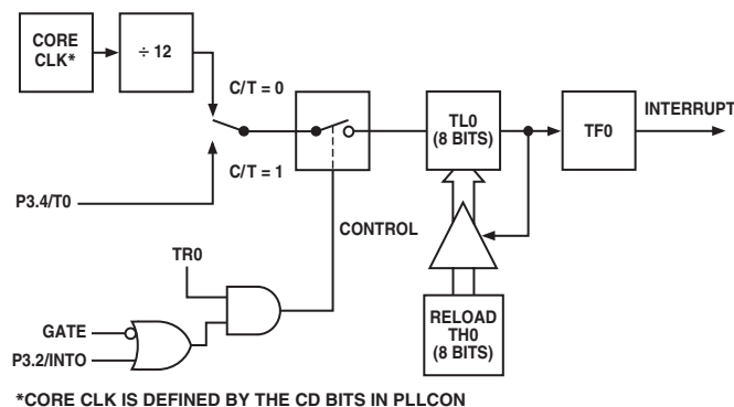
Figure 47. Timer/Counter 0, Mode 2
