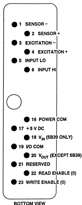
Figure 4 . Model 5B Series Module, with pin-out assignments.
