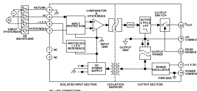
Figure 1. 5B45 & 5B46 Functional Block Diagram
