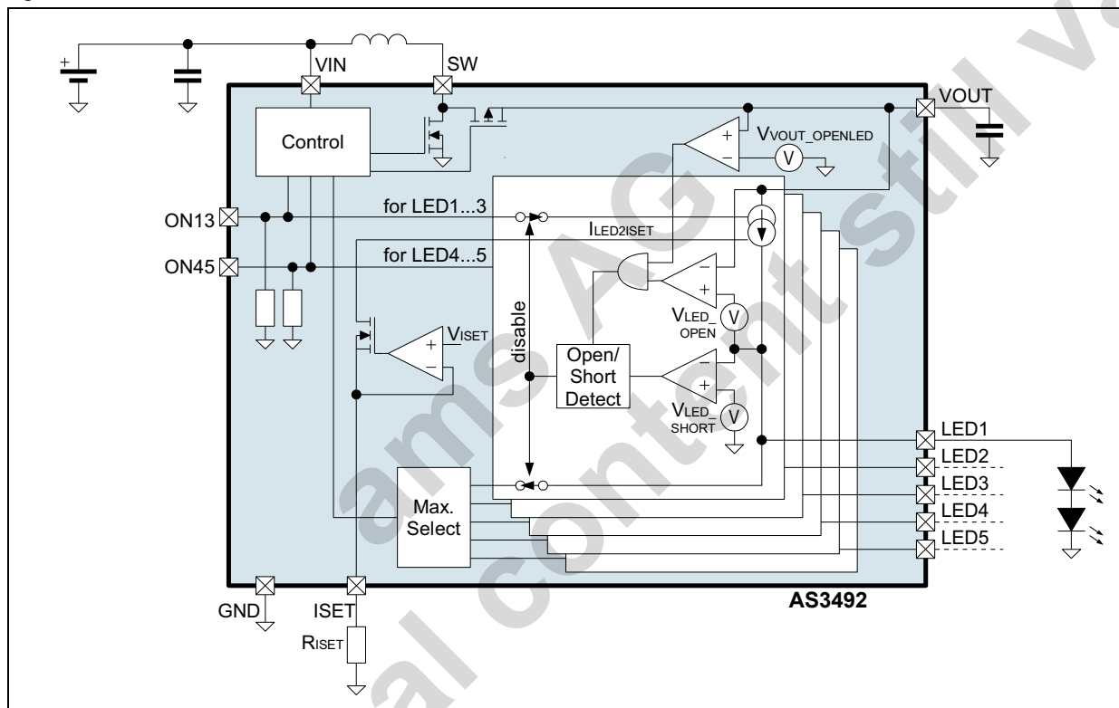
Figure 16. AS3492 internal circuit
