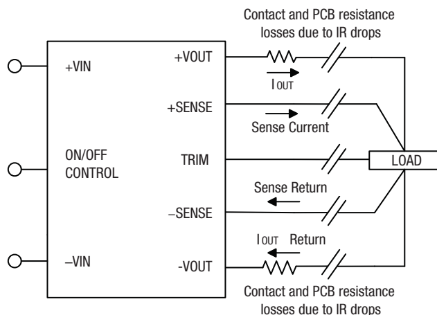
Figure 8. Remote Sense Circuit Configuration
