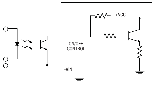
Figure 12. Driving the On/Off Control Pin (suggested circuit)
