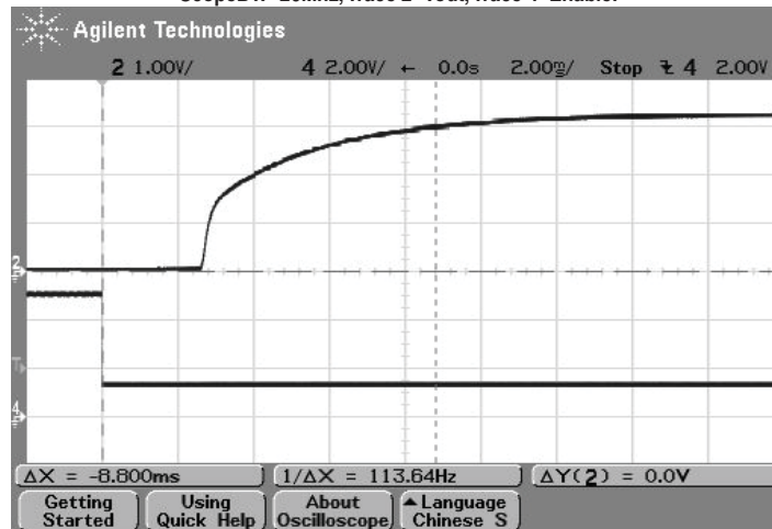
On/Off Enable Delay (Vin=48V, Vout=nom., Iout=0A, Cload=0, Ta=+25° C., ScopeBW=20Mhz, Trace 2=Vout, Trace 4=Enable.
