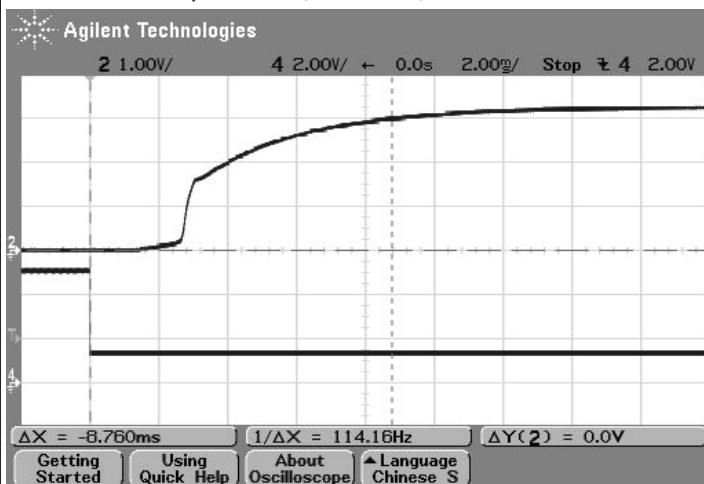
On/Off Enable Delay (Vin=48V, Vout=nom., Iout=0A, Cload=0, Ta=+25° C., ScopeBW=20Mhz, Trace 2=Vout, Trace 4=Enable.
