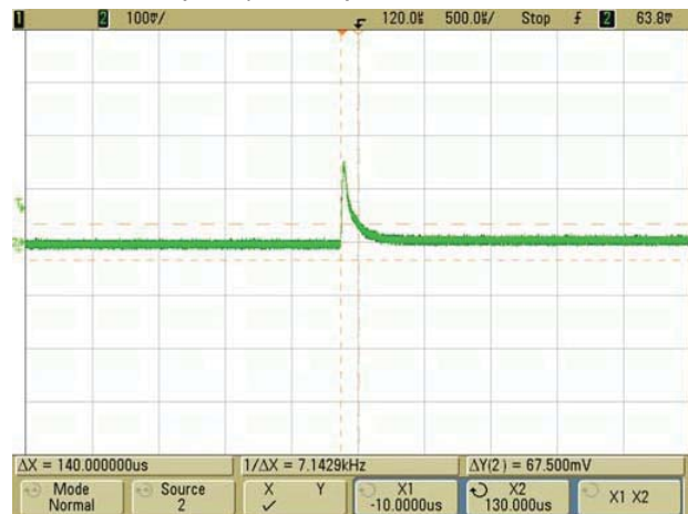
Step Load Transient Response (Slew=1A / \mu Sec., Vin=48V., Cload=0, Iout=15A to 22.5A)
