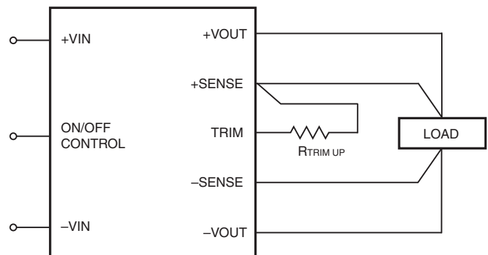
Figure 10. Trim Connections To Increase Output Voltages
