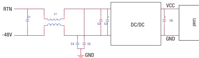
Figure 5. Conducted Emissions Test Circuit
