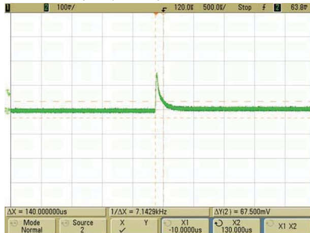
Step Load Transient Response (Slew=1A / \mu Sec., Vin=48V., Load=0, Iout=15A to 22.5A)
