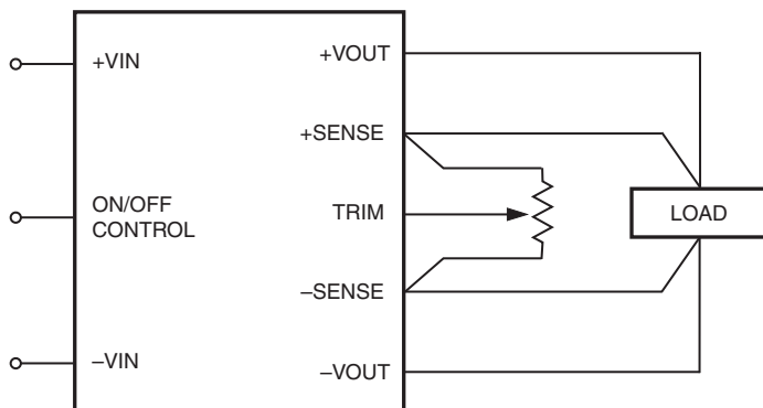
Figure 9. Trim Connections Using A Trimpot
