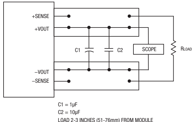
Figure 7. Measuring Output Ripple and Noise (PARD)
