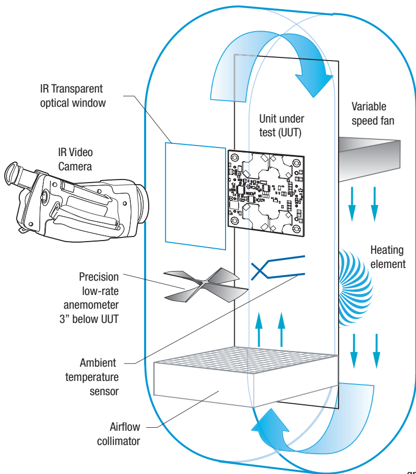
Figure 13. Vertical Wind Tunnel
