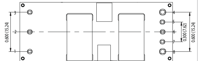
BOTTOM PIN SIDE VIEW
