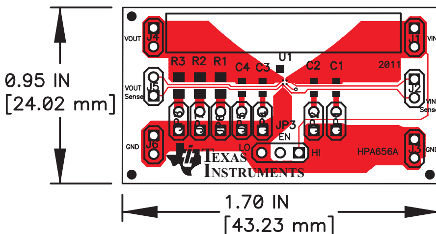
Figure 2. Top Layer
