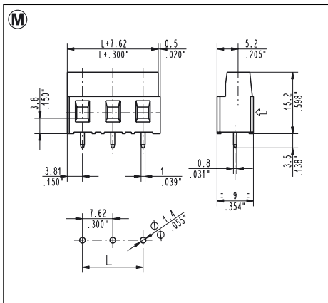
MSM_007 Straight, Side Entry 7.62 mm / .300" Pitch Weight per pole: 1.75 g
