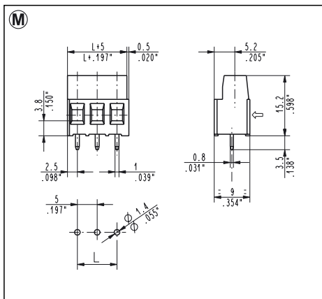
MSM_001 Straight, Side Entry 5 mm / .197" Pitch Weight per pole: 1.56 g
