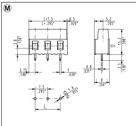
MSM_003 Straight, Side Entry 7.5 mm / .295" Pitch Weight per pole: 1.75 g
