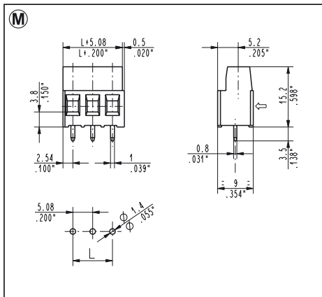
MSM_005 Straight, Side Entry 5.08 mm / .200" Pitch Weight per pole: 1.56 g
