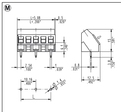
MSM_046 10.16 mm / .400" Pitch 35°, Angled Entry Weight per pole: 1.77 g
