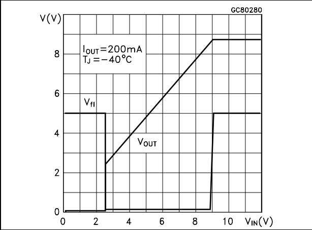
Figure 5. Output and flag voltage vs input voltage
