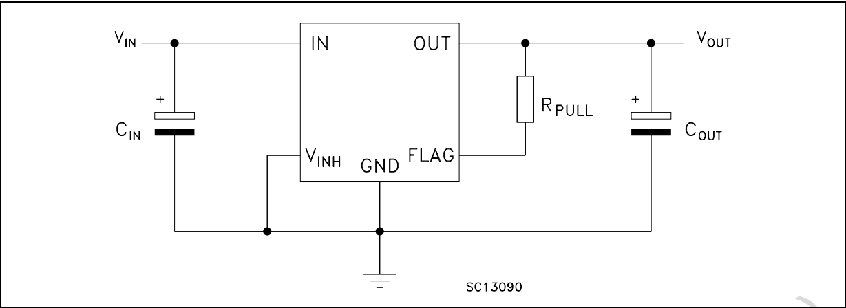
Figure 11. Test circuit
