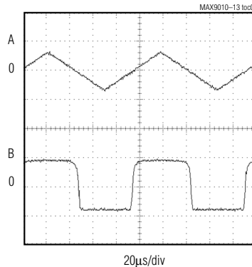
RESPONSE TO 10kHz TRIANGLE WAVE
