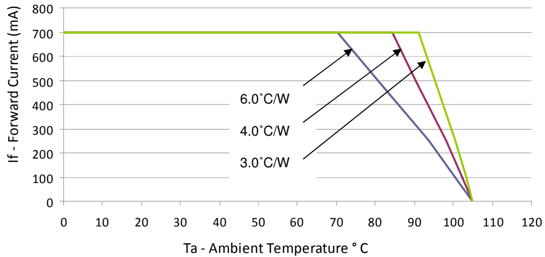
Figure 30: Derating Curve for BXRA-W0401, 700mA Drive Current
