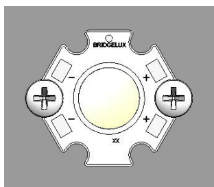
Figure 42: Recommended Mounting Locations for Hexagonal Star Products
