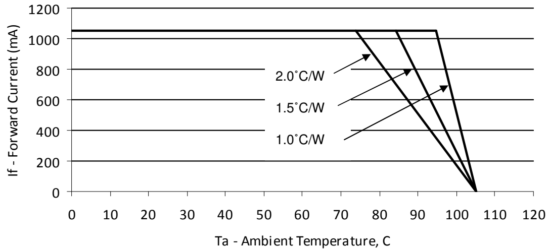
Figure 35: Derating Curve for BXRA-N1203 and BXRA-W1203, 1050 mA Drive Current
