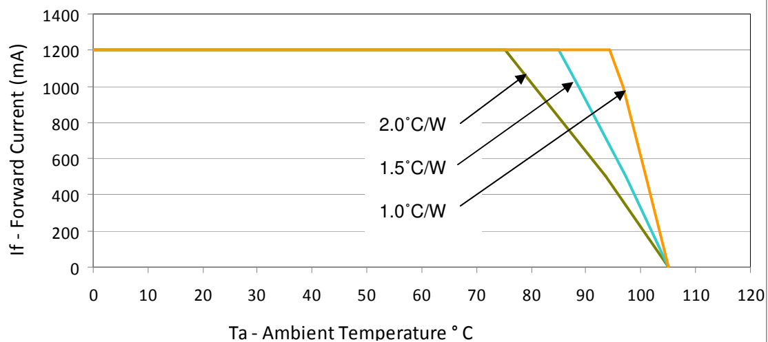
Figure 36: Derating Curve for BXRA-W1202, 1200 mA Drive Current
