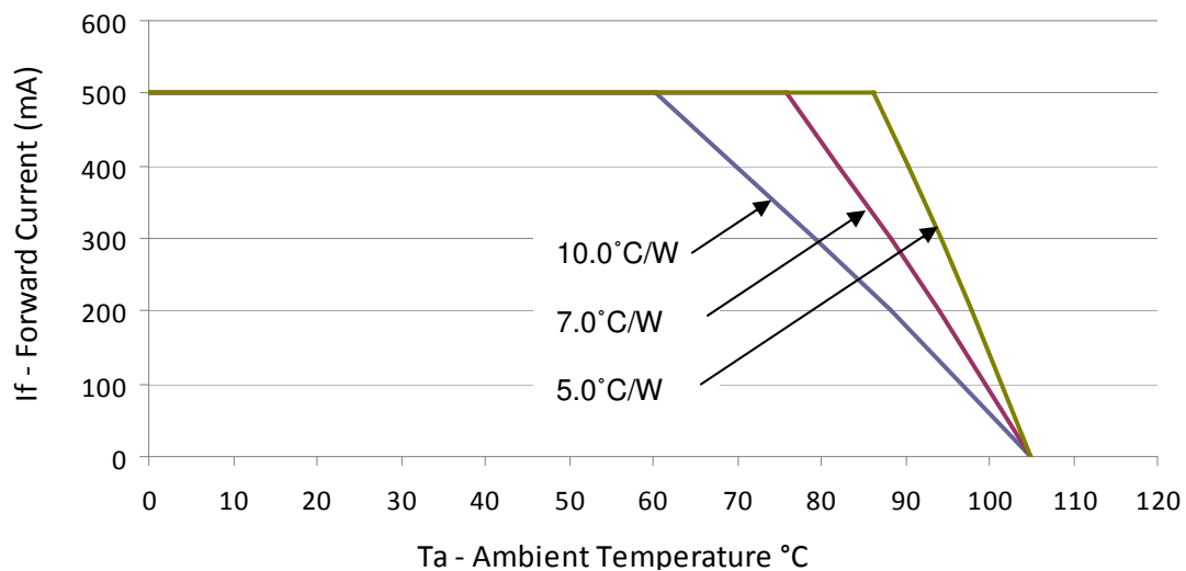
Figure 28: Derating Curve for BXRA-C0402, 500mA Drive Current
