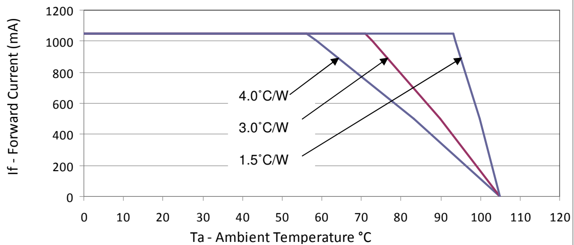
Figure 34: Derating Curve for BXRA-C1202, 1050 mA Drive Current
