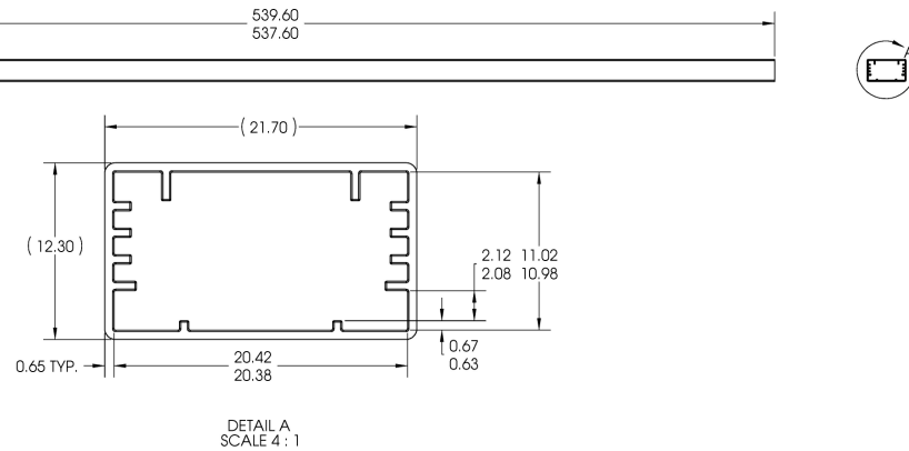
Figure 46: Tube Design for Hexagonal Star Products
