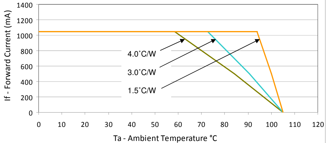
Figure 33: Derating Curve for BXRA-W0802, BXRA-N0802, 1050mA Drive Current
