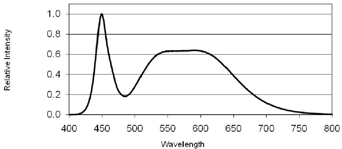
Figure 6: Typical Neutral White Color Spectrum
