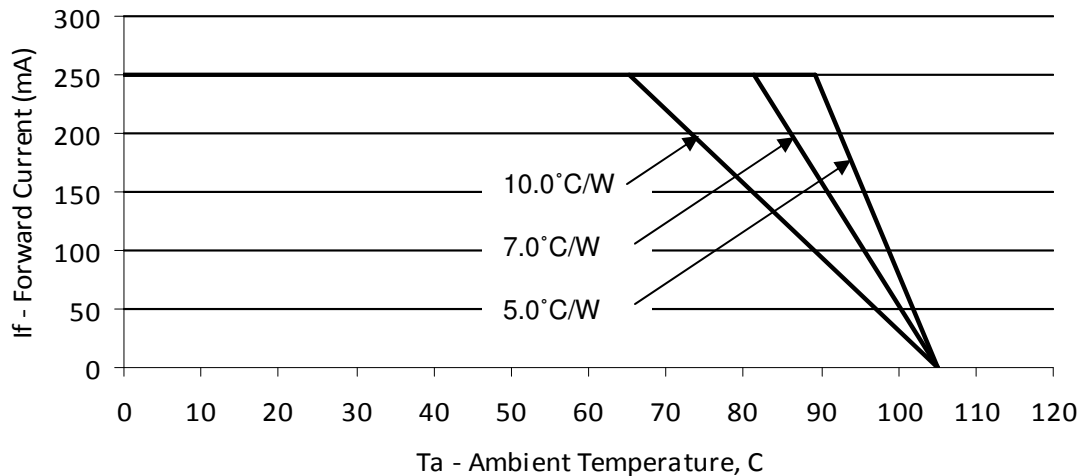
Figure 27: Derating Curve for BXRA-W0403 and BXRA-C0603, 250mA Drive Current
