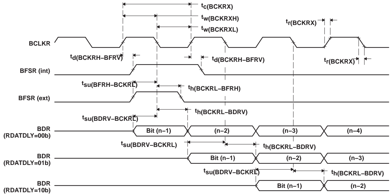
Figure 5-19. McBSP Receive Timings
