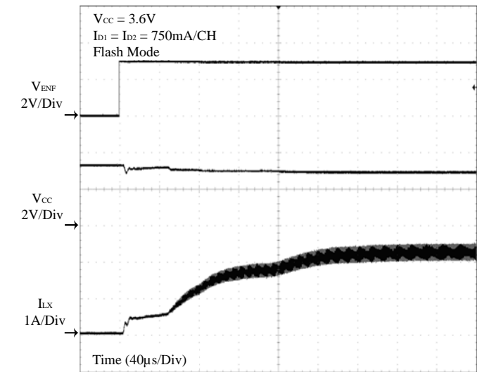
Figure 8 LX Current
