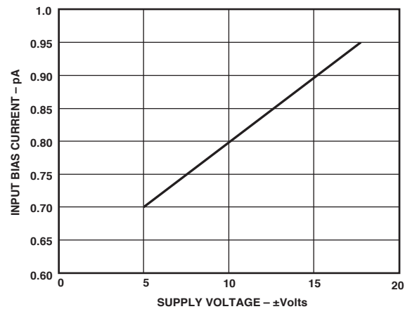
Figure 4. Input Bias Current vs. Supply
