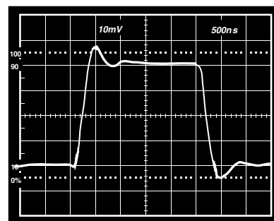
Figure 26. Unity Gain Inverter Small Signal Pulse Response
