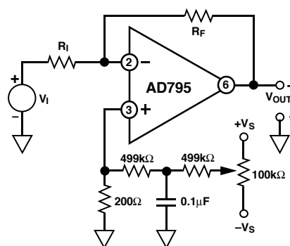
Figure 34. Alternate Offset Null Circuit for Inverter
