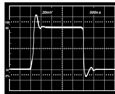
Figure 29. Unity Gain Follower Small Signal Pulse Response
