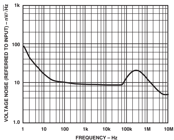
Figure 12. Input Voltage Noise Spectral Density
