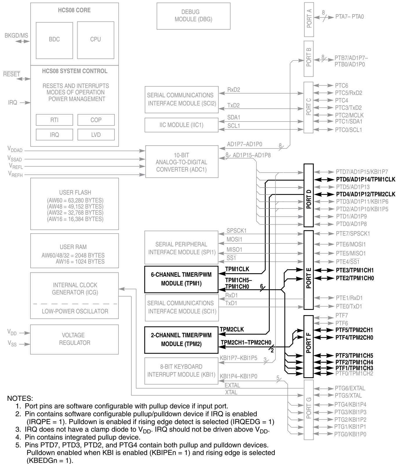
Figure 10-1. Block Diagram Highlighting the TPM Module
