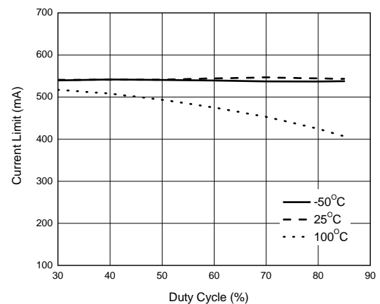
Figure 15. Current Limit vs. Duty Cycle
