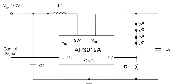
Figure 18. Typical Application Circuit to Decide R1
