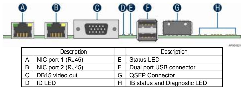
Figure 3. Rear Panel Connector Placement
