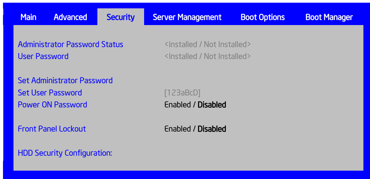
Figure 37. Security Screen
