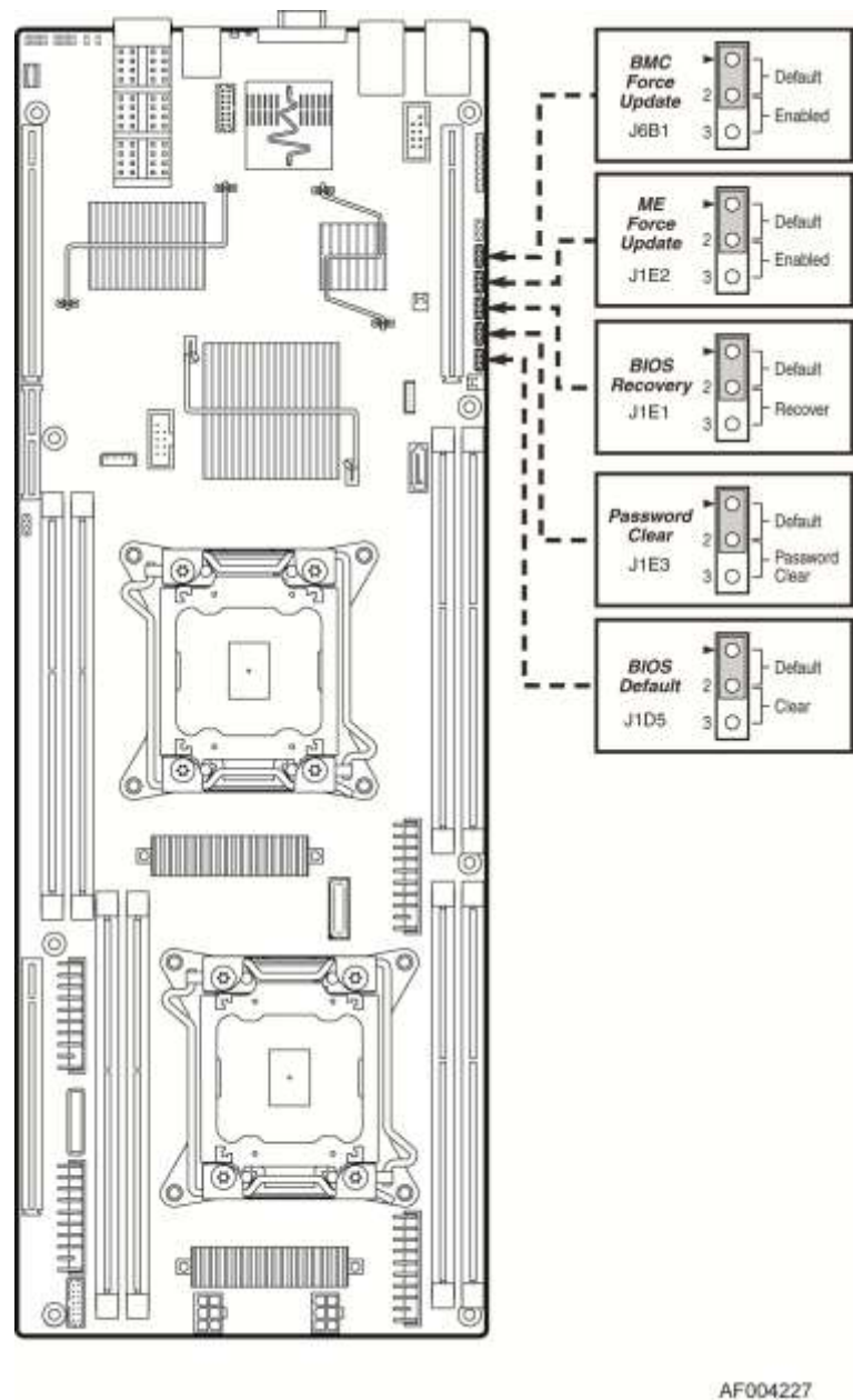
Figure 48. Jumper Blocks (J6B1, J1E2, J1E3, J1E1, and J1D5)
