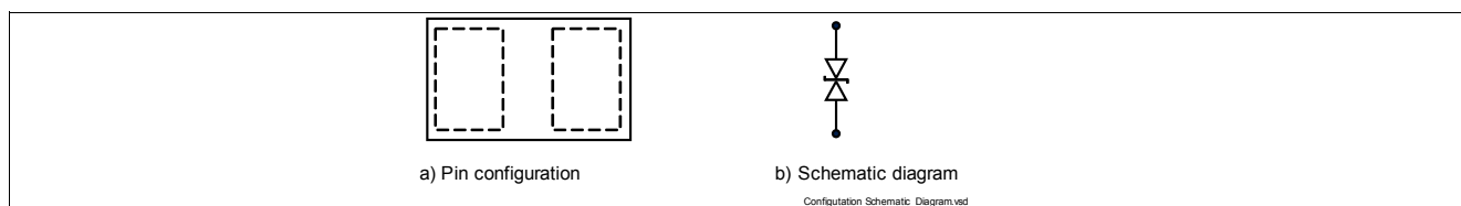
Figure 1-1 Pin Configuration and Schematic Diagram
