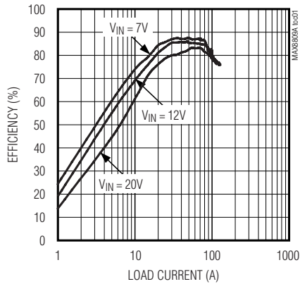
EFFICIENCY vs. LOAD CURRENT R_{SC} = 130k\Omega
