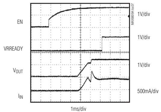
SOFT-START WAVEFORMS (INTEL)
