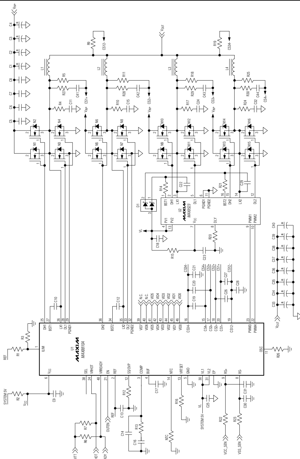
Figure 15. AMD K8 Rev F Desktop Application Circuit Using the MAX8810A—4-Phase, 115A
