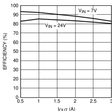
Figure 7-10. Demoboard Efficiency
