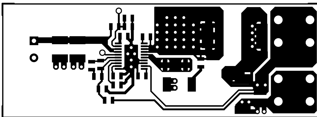
Figure 7-11. Component Side
