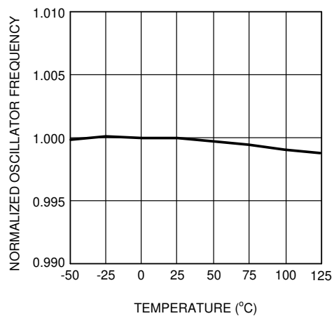
Figure 5-2. Oscillator Frequency vs Temperature
