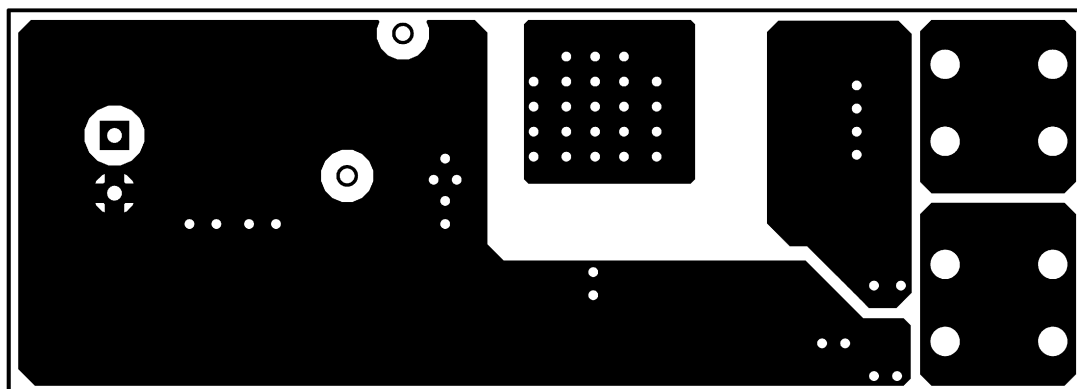
Figure 7-12. Solder Side
