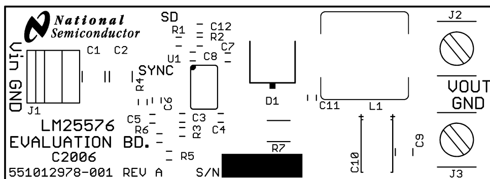
Figure 7-13. Silkscreen
