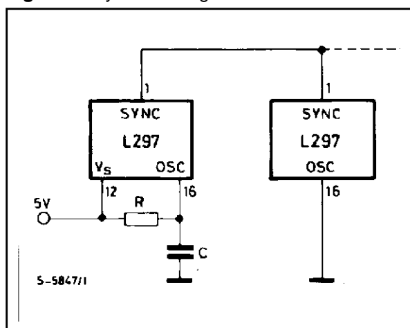
Figure 3 : Synchronising L297s
