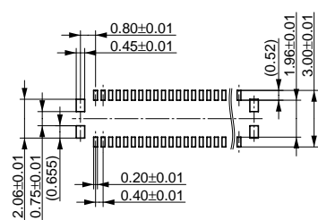
Recommended metal mask opening pattern Metal mask thickness: When 120μm (Terminal opening ratio: 60%) (Metal-part opening ratio: 100%)
