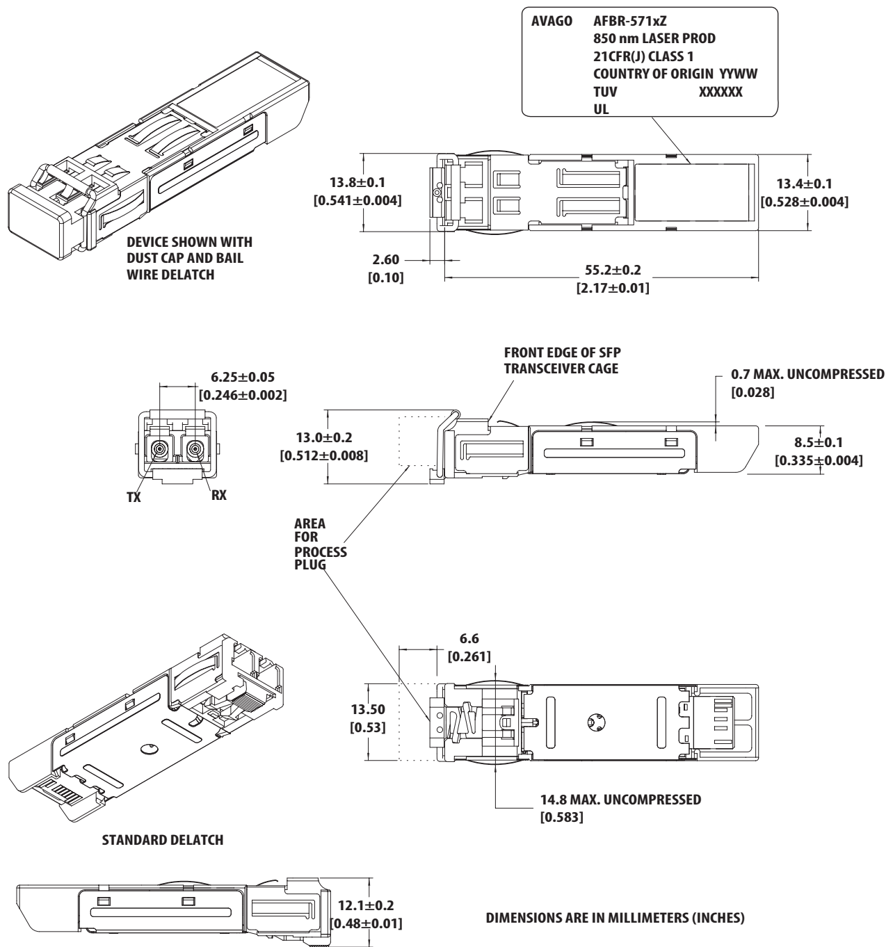
Figure 7. Module drawing
