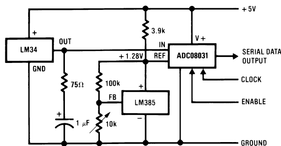
Figure 23. Temperature-to-Digital Converter (Serial Output, 128°F Full Scale)
