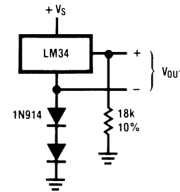
Figure 17. Full Range Fahrenheit Sensor ( -50^\circ\text{F} to 300^\circ\text{F} )
