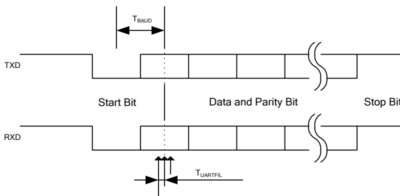
Figure 11. UART timing
