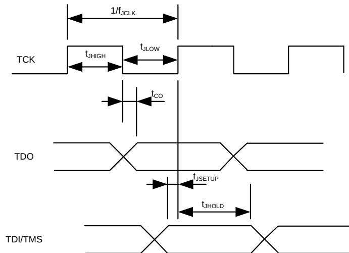
Figure 13. JTAG timing
