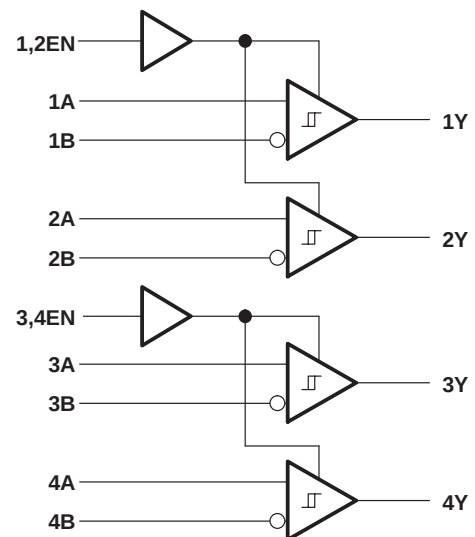
logic diagram
