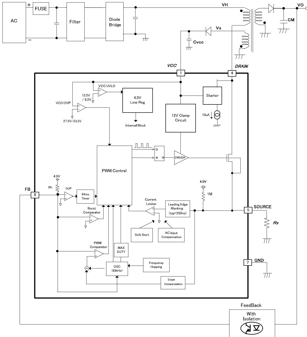
Figure 3. Block Diagram
