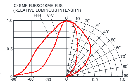
FIG.6b RED FAR FIELD PATTERN
