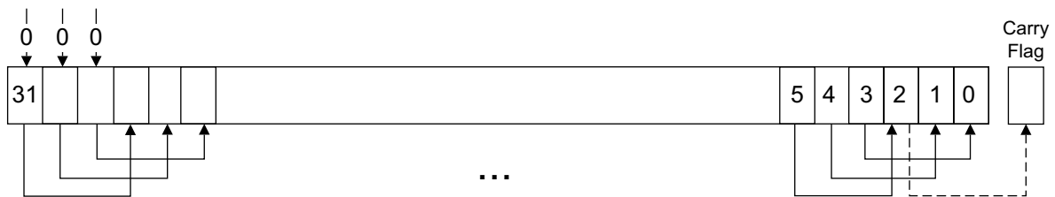
Fig 50. LSR #3
