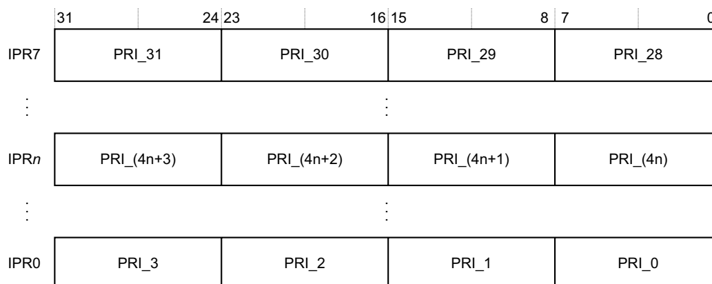
Fig 53. IPR register
