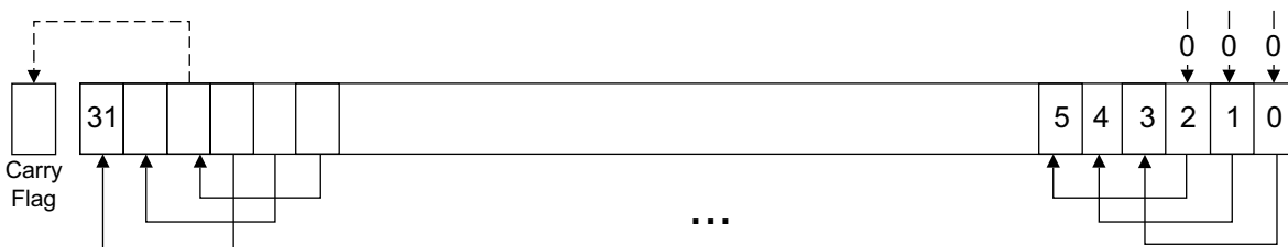
Fig 51. LSL #3
