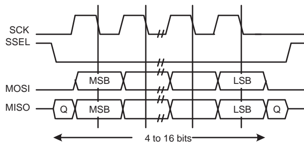
Fig 18. SPI frame format with CPOL=0 and CPHA=1
