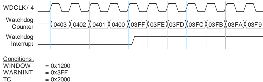
Fig 35. Watchdog Warning Interrupt
