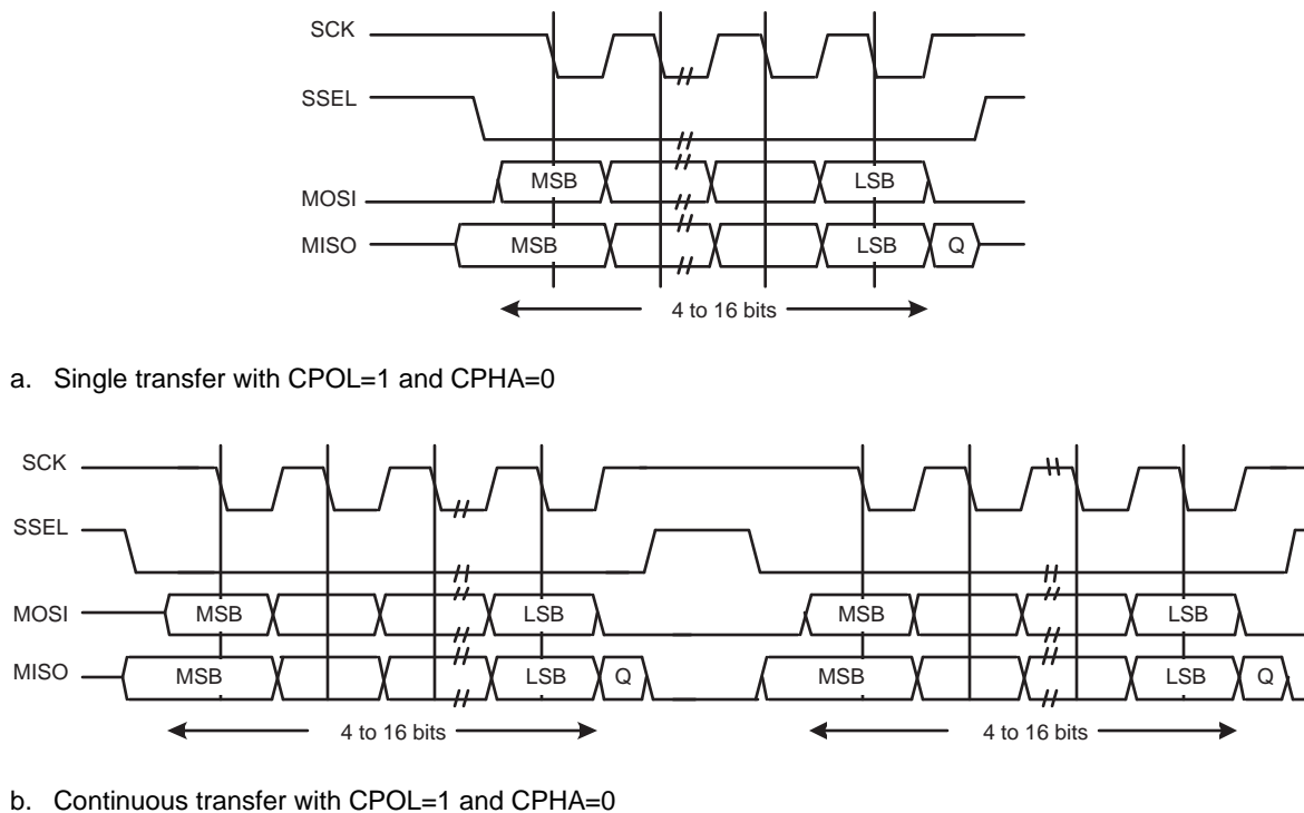
Fig 19. SPI frame format with CPOL = 1 and CPHA = 0 (a) Single and b) Continuous Transfer)
