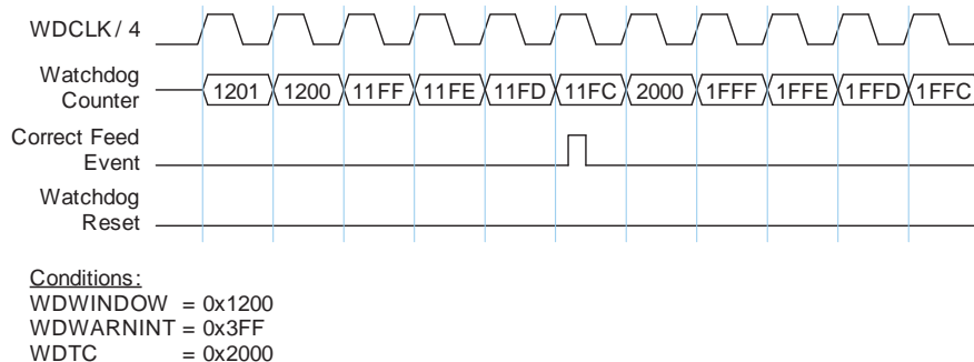
Fig 34. Correct Watchdog Feed with Windowed Mode Enabled
