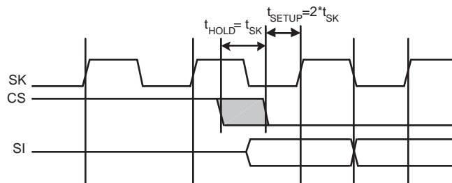
Fig 23. Microwire frame format setup and hold details
