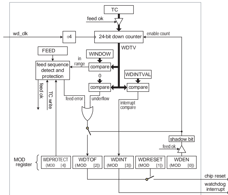
Fig 32. Windowed Watchdog Timer (WWDt) block diagram
