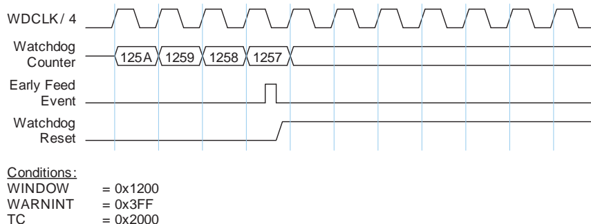
Fig 33. Early Watchdog Feed with Windowed Mode Enabled
