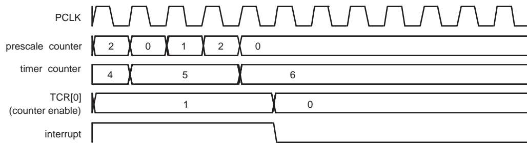
Fig 30. A timer cycle in which PR=2, MRx=6, and both interrupt and stop on match are enabled
