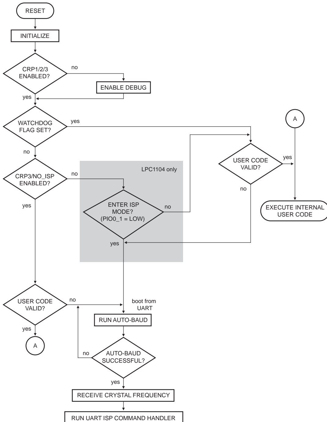
Fig 37. Boot process flowchart
