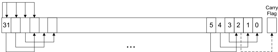
Fig 49. ASR #3
