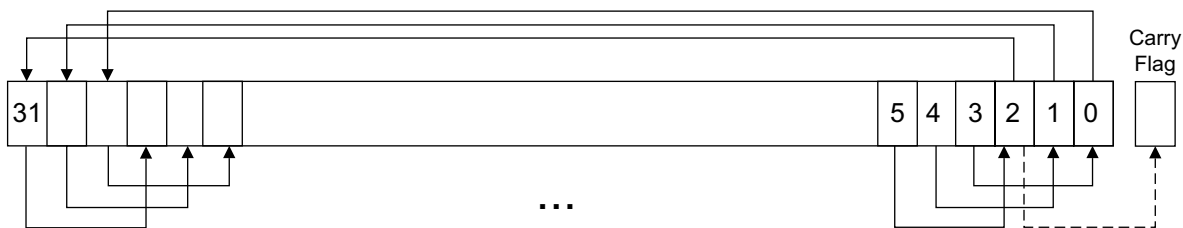
Fig 52. ROR #3
