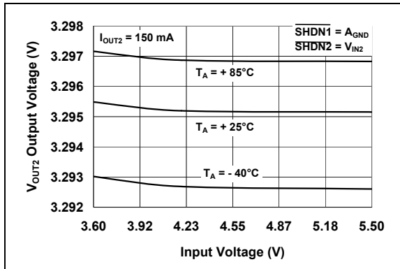
FIGURE 2-25: V_{OUT2} Output Voltage vs. Input Voltage ( V_{OUT2} = 3.3V ).
