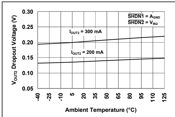
FIGURE 2-26: V_{OUT2} Dropout Voltage vs. Ambient Temperature ( V_{OUT2} = 2.5V ).
