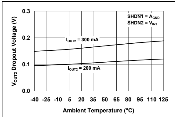
FIGURE 2-27: V_{OUT2} Dropout Voltage vs. Ambient Temperature ( V_{OUT2} = 3.3V ).
