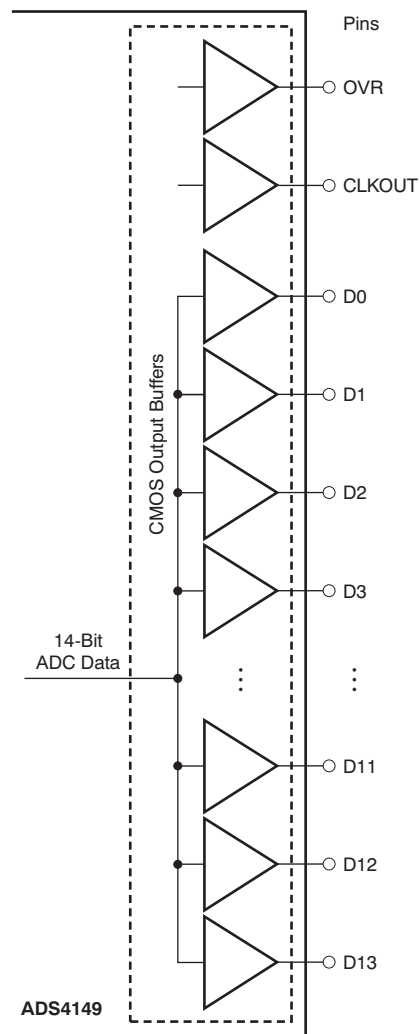
Figure 128. CMOS Output Interface
